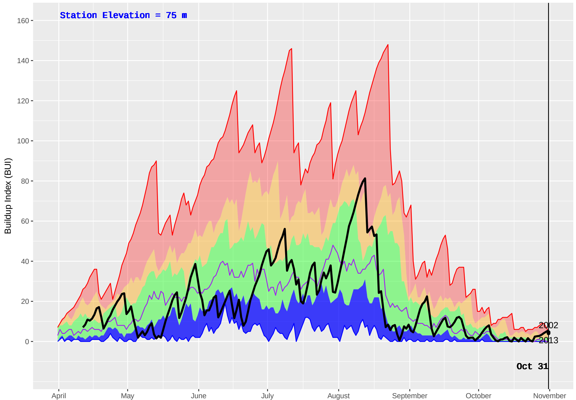
KITPARK (106) : Historical (1995–2016) and Current (2017) Noon Buildup Index (BUI)
