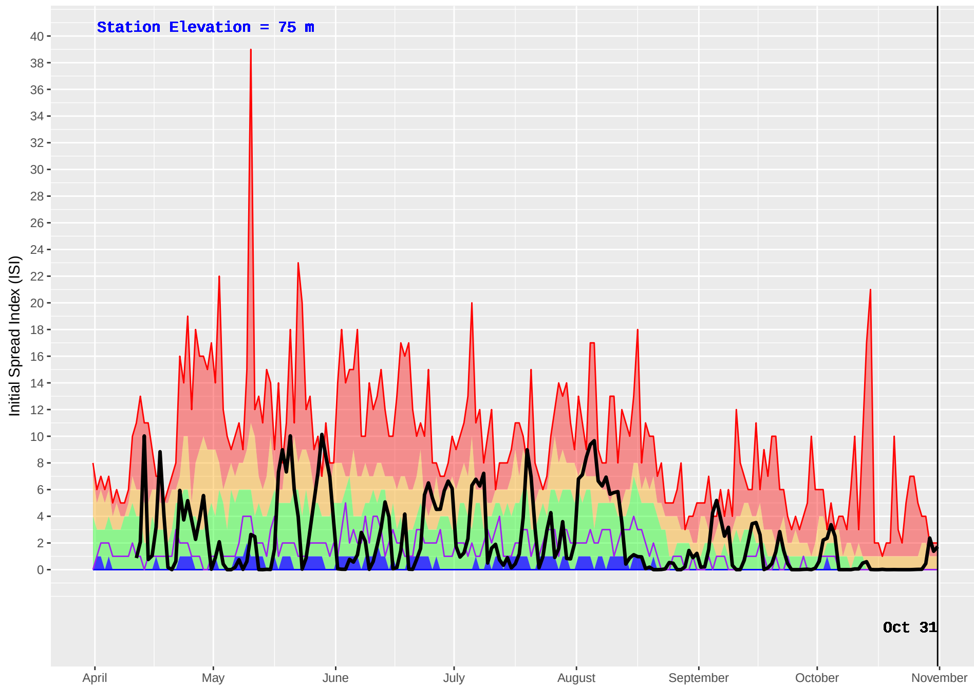
KITPARK (106) : Historical (1995–2016) and Current (2017) Noon Initial Spread Index (ISI)
