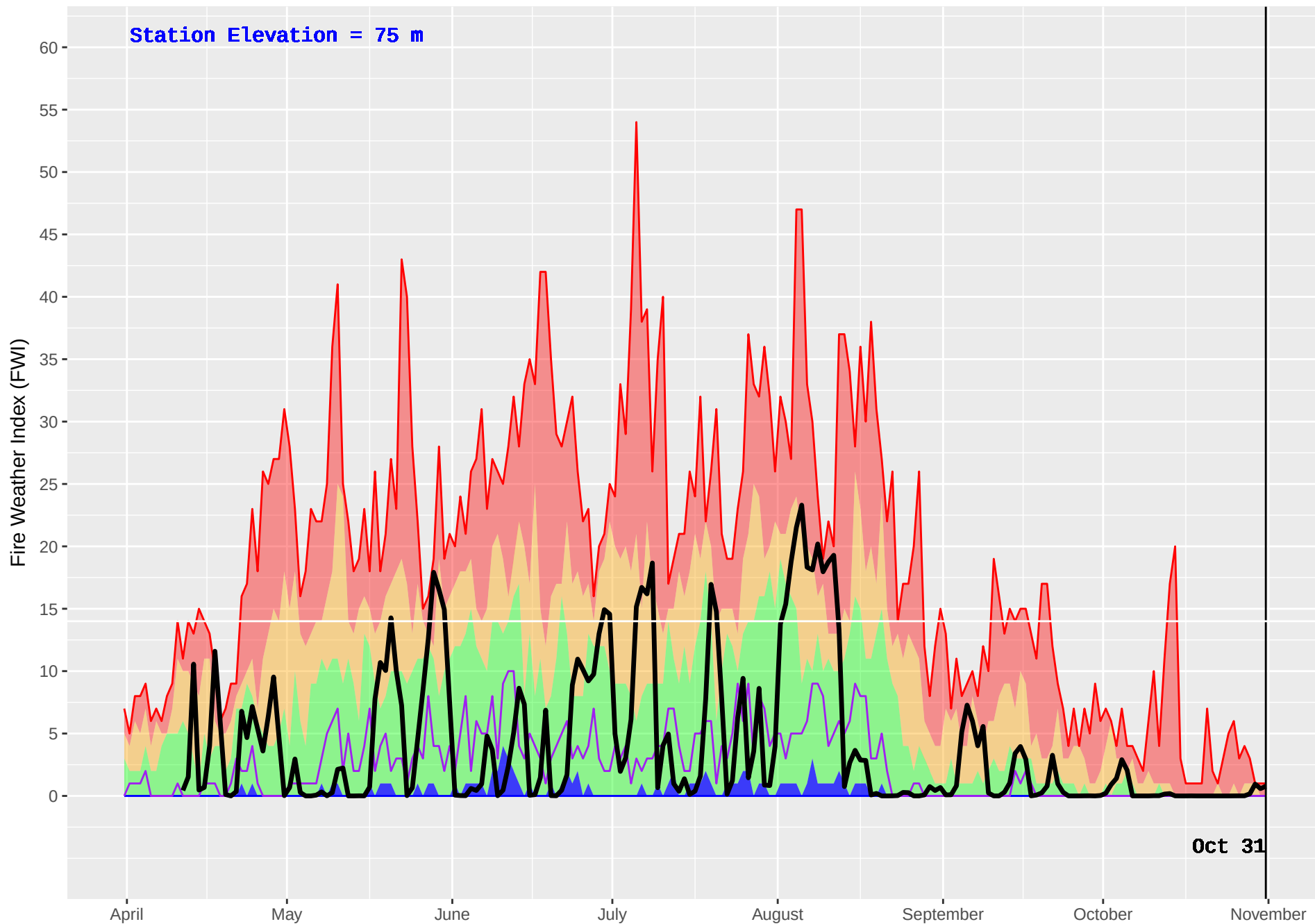
KITPARK (106) : Historical (1995–2016) and Current (2017) Noon Fire Weather Index (FWI)
