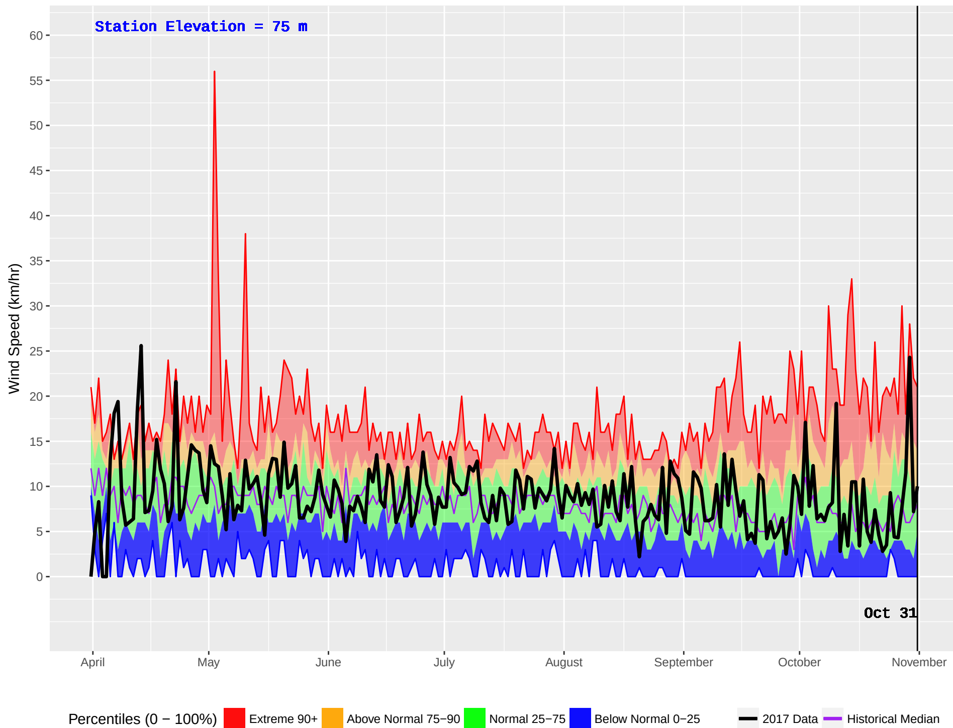
KITPARK (106) : Historical (1995–2016) and Current (2017) Noon Wind Speed
