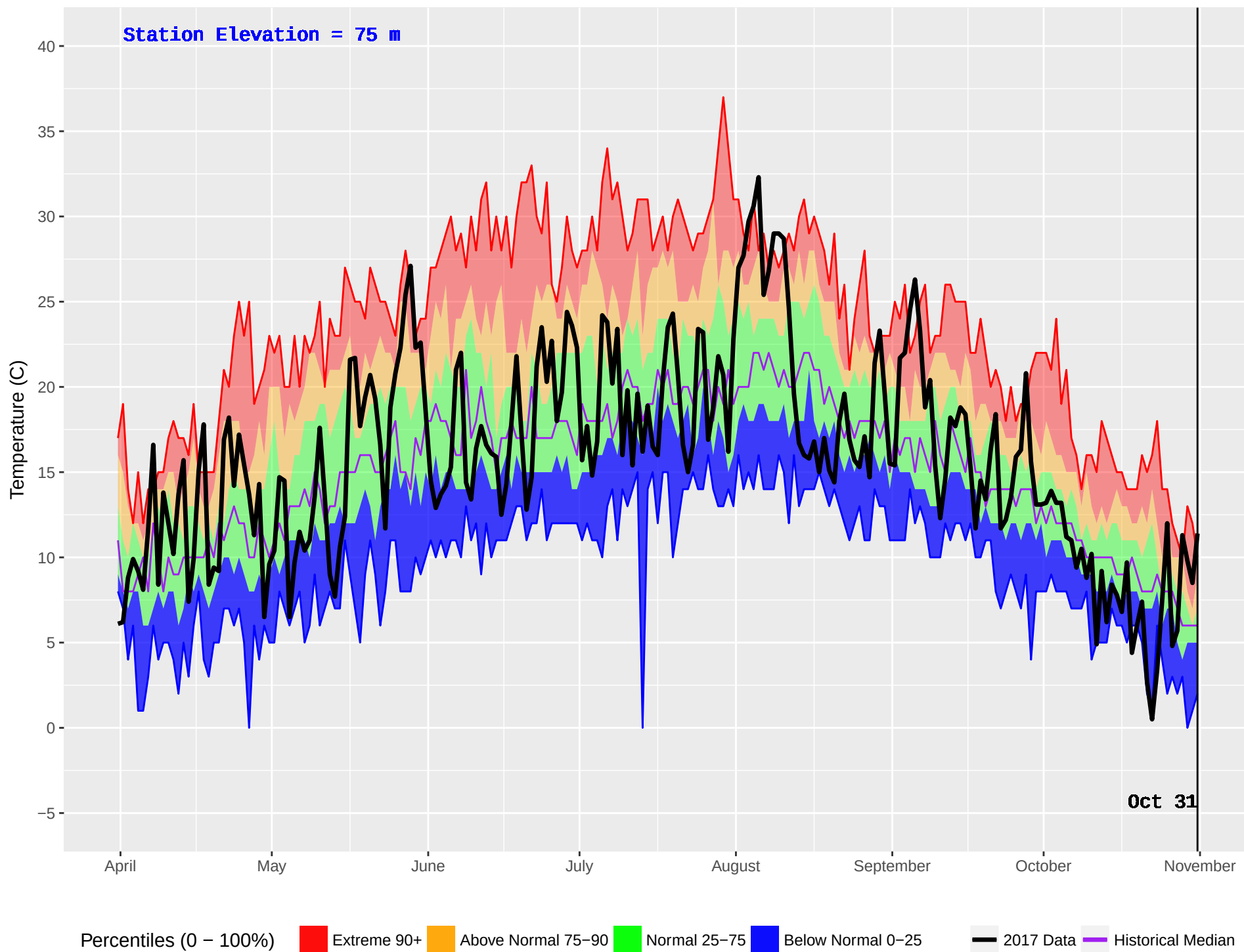
KITPARK (106) : Historical (1995–2016) and Current (2017) Noon Temperature
