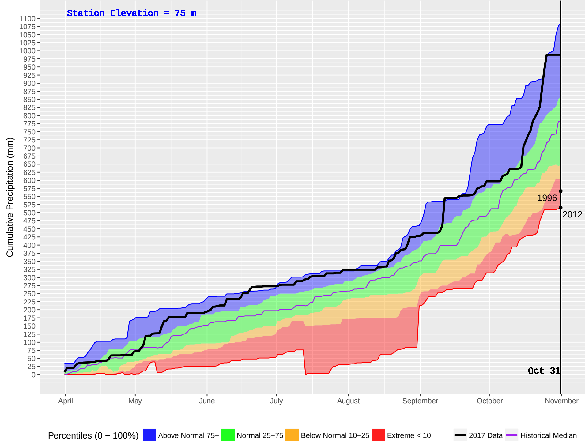
KITPARK (106) : Historical (1995–2016) and Current (2017) Noon Cumulative Precipitation
