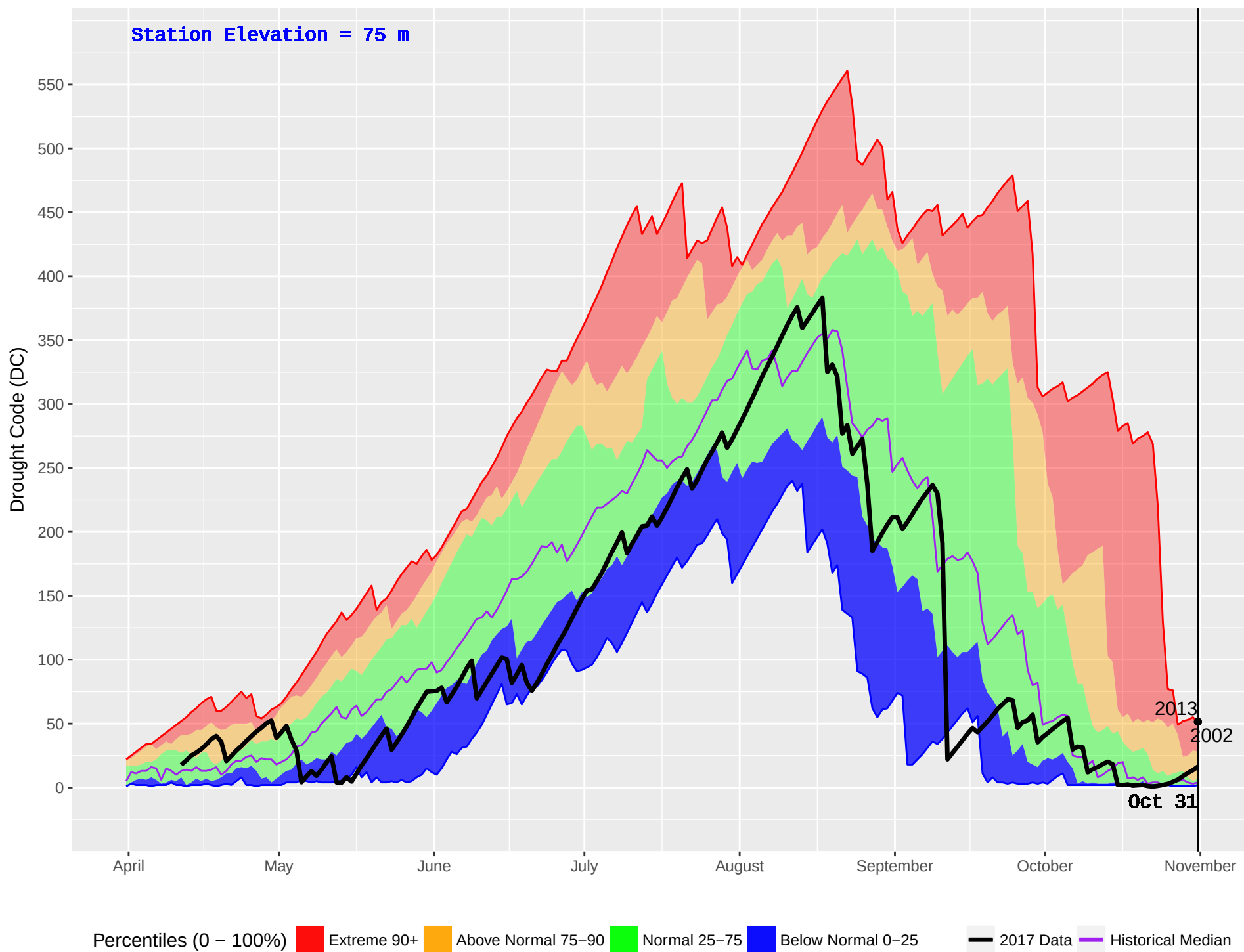
KITPARK (106) : Historical (1995–2016) and Current (2017) Noon Drought Code (DC)
